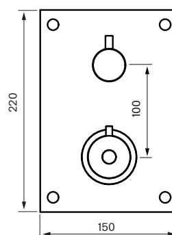
Mixer front view
