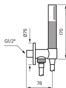
Hand shower
